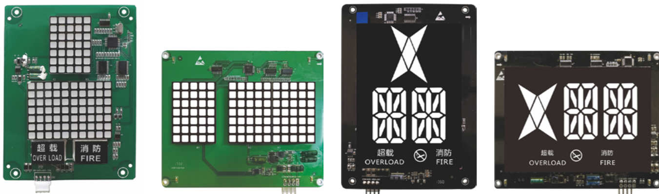
GNL-DOT-64 • 6.4 INCH DOT DISPLAY • INSTALL SIZE:160*105MM- 安装尺寸 • FACEPLATE:140*80MM - 面板尺寸 GNL-DOT-64-HZ • 6.4 INCH DOT DISPLAY • INSTALL SIZE:129*147MM- 安装尺寸 • FACEPLATE:94*129MM - 面板尺寸 GNL-LED-64 • 6.4 INCH DOT DISPLAY • INSTALL SIZE:160*106MM- 安装尺寸 • FACEPLATE:130*95MM - 面板尺寸 GNL-LED-64-HZ • 6.4 INCH DOT DISPLAY • INSTALL SIZE:94*130MM - 安装尺寸 • FACEPLATE:95*130MM - 面板尺寸
