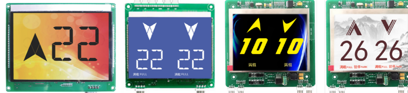
GNL-CBLCD-64-HZ • 6.4 INCH LCD DISPLAY • INSTALL SIZE:94*131MM - 安装尺寸 • FACEPLATE:95*131MM - 面板尺寸 GNL-LCD-64-DPLX • 6.4 INCH LCD DISPLAY • INSTALL SIZE:115*120MM- 安装尺寸 • FACEPLATE:86*115MM - 面板尺寸 GNL-HD-56-DPLX-BLU • 5.6 INCH HD DUPLEX DISPLAY • INSTALL SIZE:115*120MM- 安装尺寸 • FACEPLATE:87*115MM - 面板尺寸 GNL-HD-56-DPLX-WIT • 5.6 INCH HD DUPLEX DISPLAY • INSTALL SIZE:115*120MM- 安装尺寸 • FACEPLATE:87*115MM - 面板尺寸
